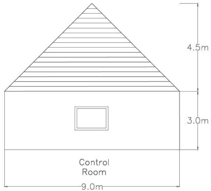
SOUTH ELEVATION
