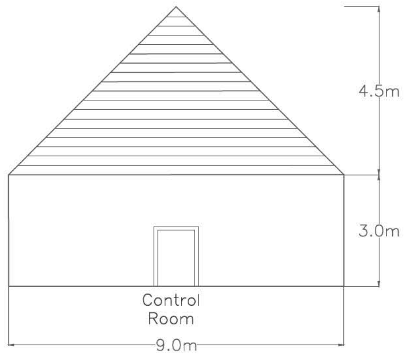
NORTH ELEVATION
