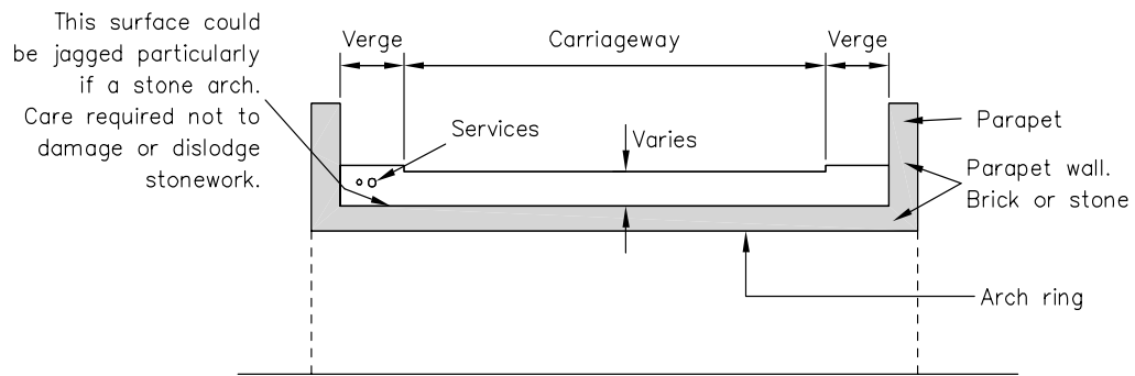
CROSS SECTION (No concrete saddle or waterproofing)
