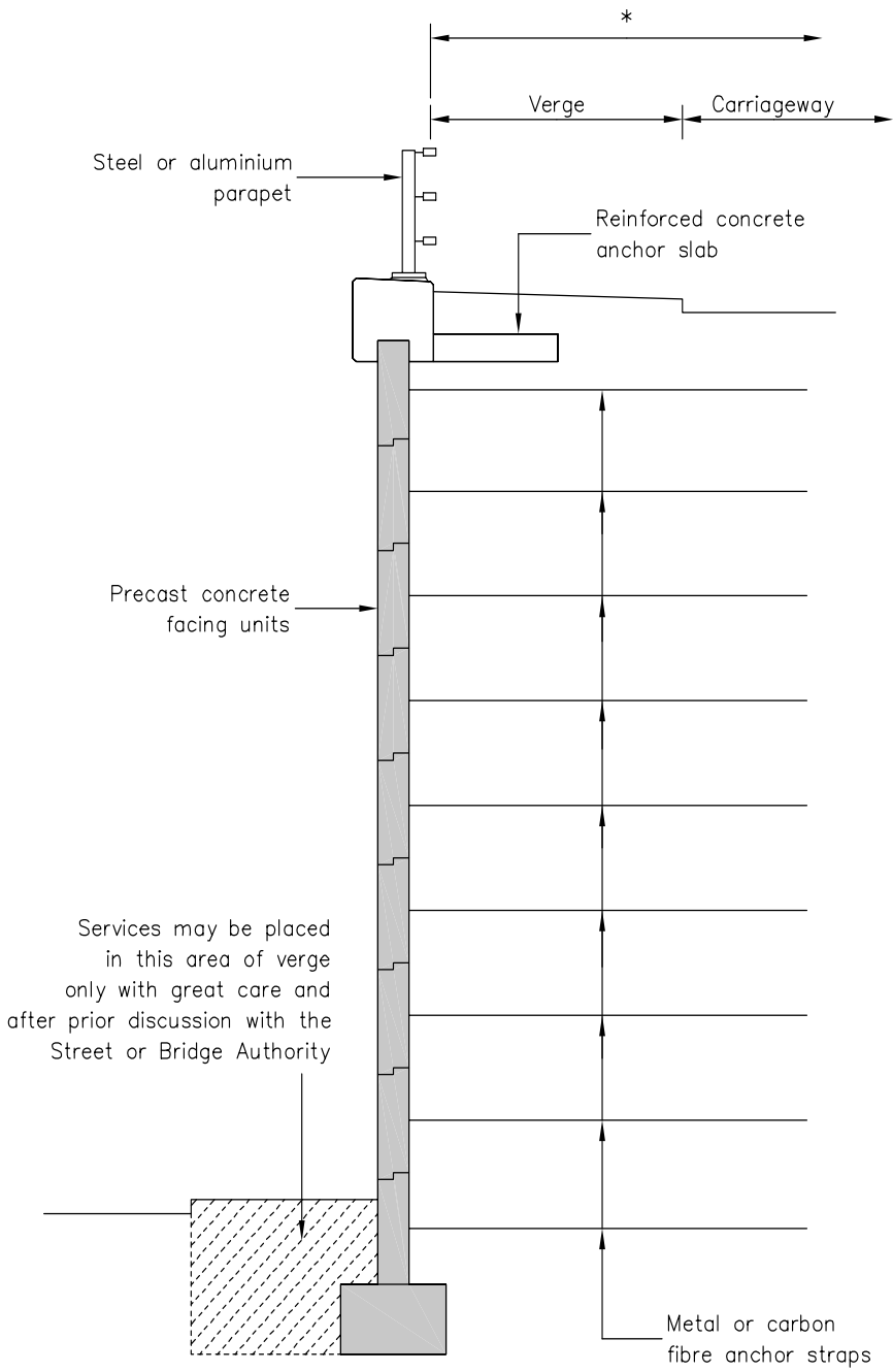
Fig 8 TYPICAL REINFORCED EARTH RETAINING WALL Not to scale
