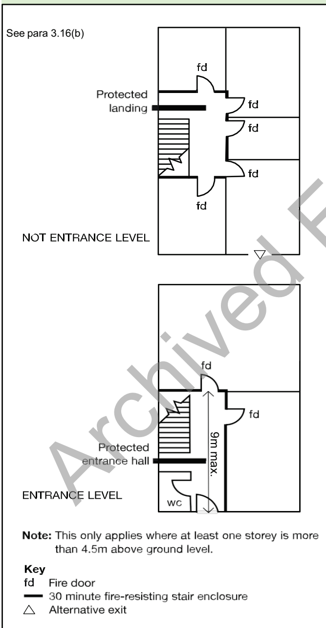
Diagram 6 Multi-storey flat with protected entrance hall and
