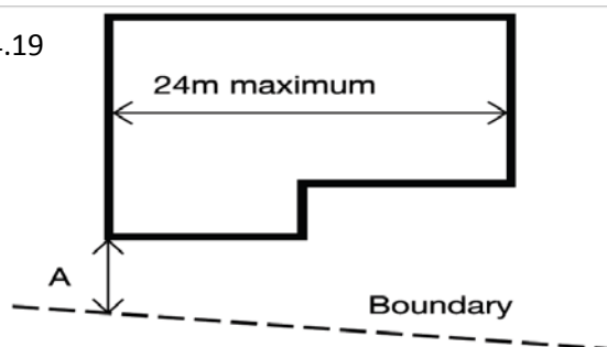
Diagram 46 Permitted unprotected areas in small residential buildings
