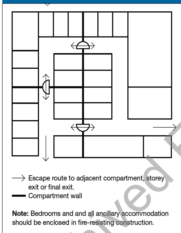
Diagram 19 Progressive horizontal evacuation in care homes
